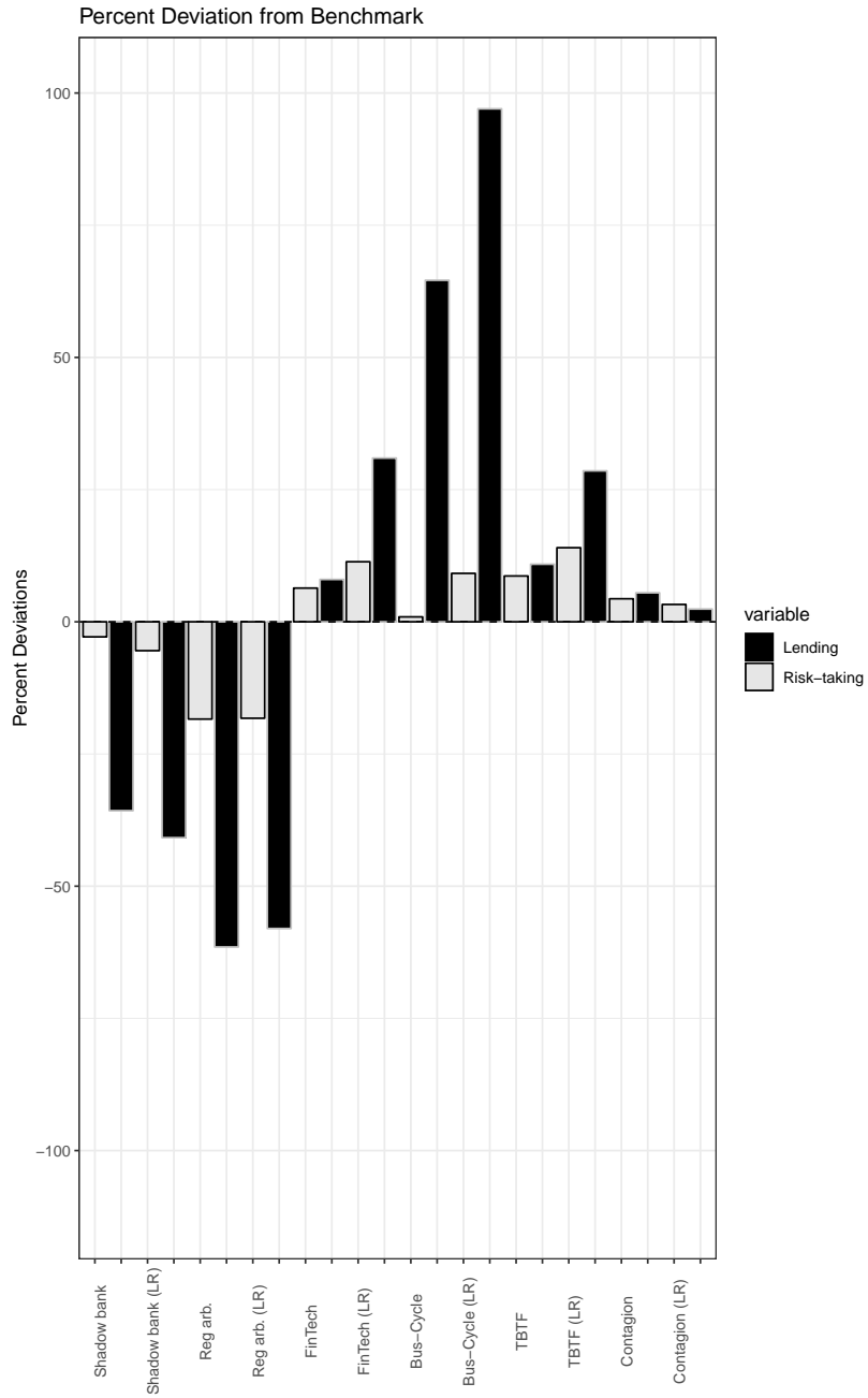
Figure 7: Robustness
